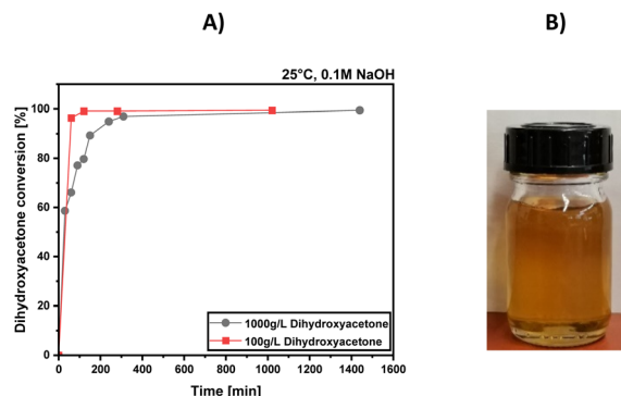
Fig. 1 (A) Consumption of dihydroxyacetone over time at a 100 g per L substrate loading (red curve) and 1000 g per L substrate loading (black curve) (B) physical appearance of the produced dendroketoise.
