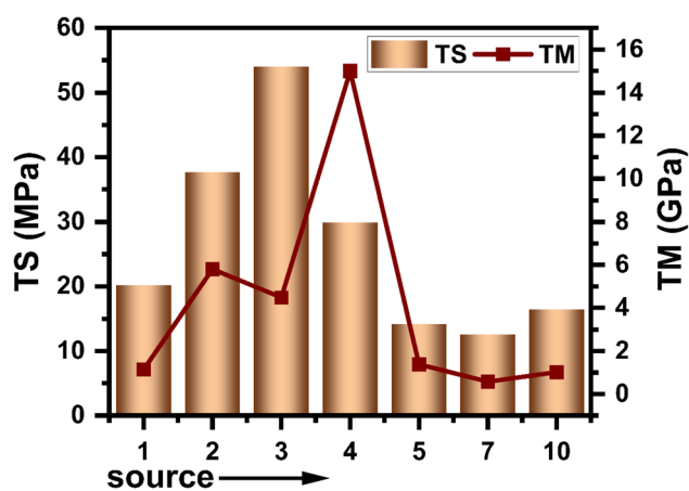
Fig. 22 Tensile properties of PS-based WPCs.
