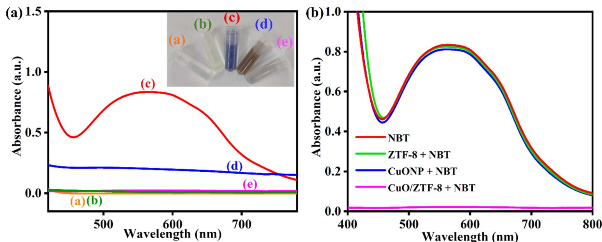
Fig. 3 Absorbance spectra of (a) \text{O}_2^{\cdot-} in DMSO (orange), (b) 1 mg \text{mL}^{-1} of NBT in 0.1 M PBS (pH 7) (green), (c) \text{O}_2^{\cdot-} -NBT system (red), (d) 0.5 mg \text{mL}^{-1} of CuO/ZTF-8 in 0.1 M PBS (pH 7) (blue), and (e) \text{O}_2^{\cdot-} -NBT system in the presence of CuO/ZTF-8 (pink). (Inset) Visual representation of the colour changes observed (b) \text{O}_2^{\cdot-} -NBT system in the absence (red) and presence of ZTF-8 (green), CuONP (blue), and CuO/ZTF-8 (pink) in 0.1 M PBS (pH 7).
