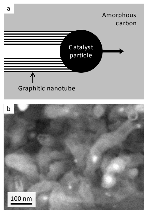
Figure 1 a) schematic showing proposed mechanism of iron-catalysed graphitization and b) scanning electron microscope image of graphitic nanotubes produced by iron-catalysed graphitization of softwood (image reproduced with permission from reference 13 )
