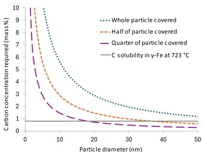
Figure 8 Estimation of carbon concentration required to cover a catalyst sphere with a single-atom thick layer of graphene.
