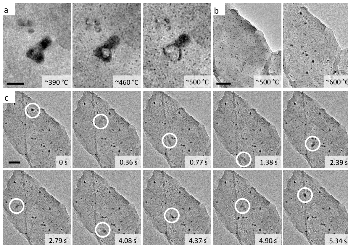
Figure 3 Snapshots from in situ TEM videos showing heating of a cellulose + \text{FeCl}_3 sample a) up to 500 °C (scale bar = 50 nm), b) from 500 °C to 600 °C (scale bar = 100 nm) and c) held at 600 °C (scale bar = 100 nm). Circles show the positions of a single particle as it moves.
