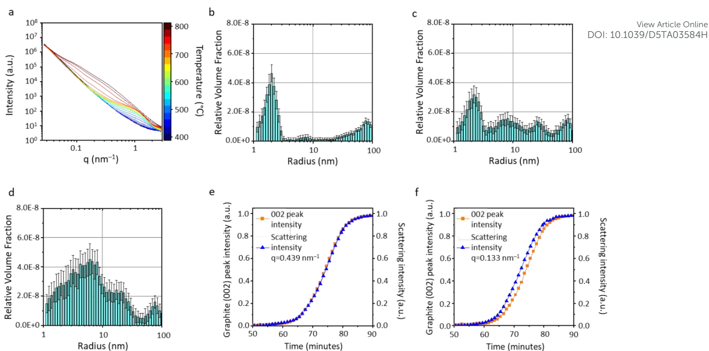
Figure 5 a) SAXS data for the heating range 400-800 °C and corresponding particle size histograms for data scans at b) 700 °C, c) 750 °C and d) 800 °C for cellulose-Fe(NO 3 ) 3 . Normalised graphite (002) peak intensity alongside scattering intensity at e) q=0.439 \text{ nm}^{-1} and f) q=0.133 \text{ nm}^{-1} .
