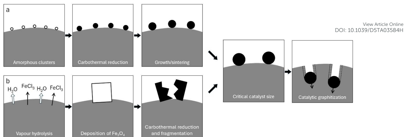
Figure 7 Schematic showing the two proposed mechanisms of graphitization catalyst formation from cellulose with a) \text{Fe}(\text{NO}_3)_3 and b) \text{FeCl}_3 .
