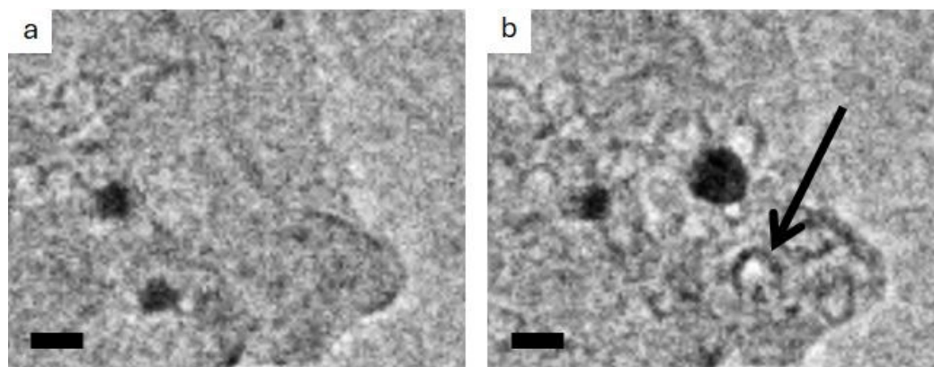
Figure 4 Snapshots from TEM video showing a region of the cellulose-FeCl 3 sample during the graphitization step, showing a) amorphous carbon with some Fe nanoparticles and b) a trail of graphitic carbon nanotubes left by a moving catalyst particle. Scale bar = 20 nm.
