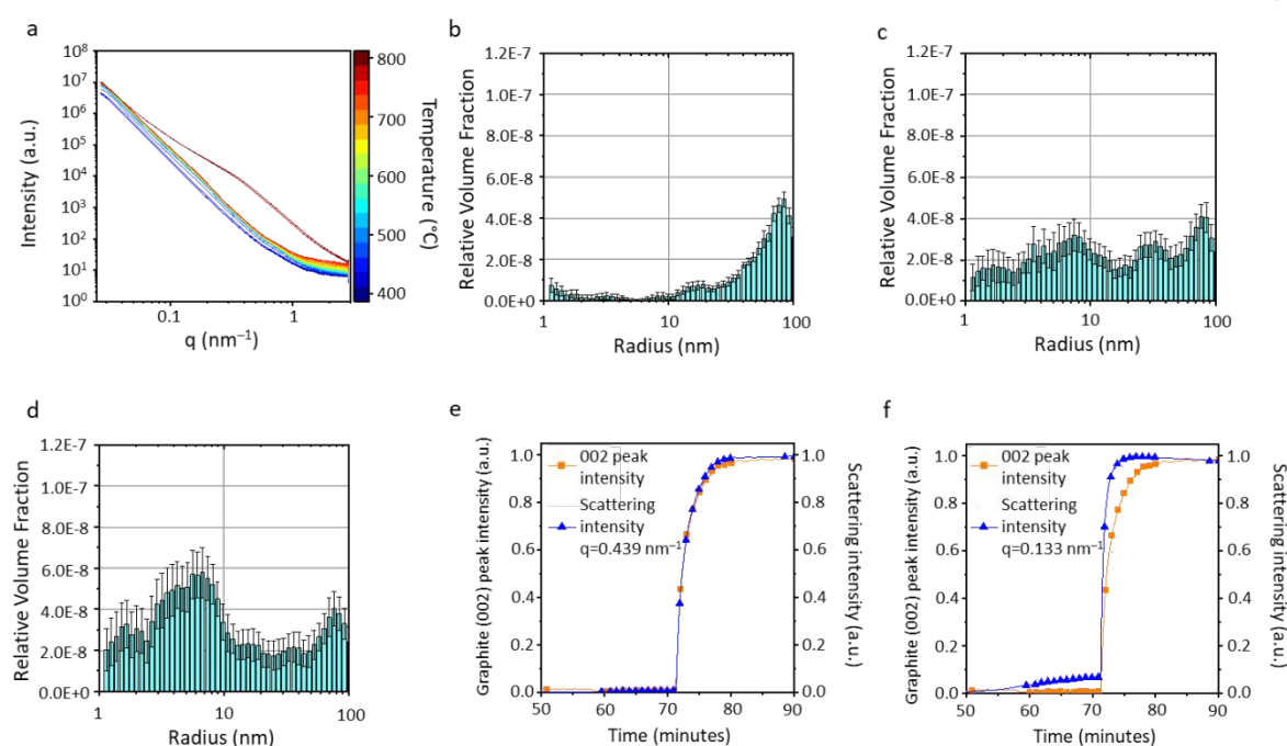
Figure 6 a) SAXS data for the heating range 400–800 °C and corresponding particle size histograms for data at b) 750 °C, c) 760 °C and d) 770 °C for cellulose- \text{FeCl}_3 . Normalised graphite (002) peak intensity alongside scattering intensity at e) q=0.439 \text{ nm}^{-1} and f) q=0.133 \text{ nm}^{-1} .
