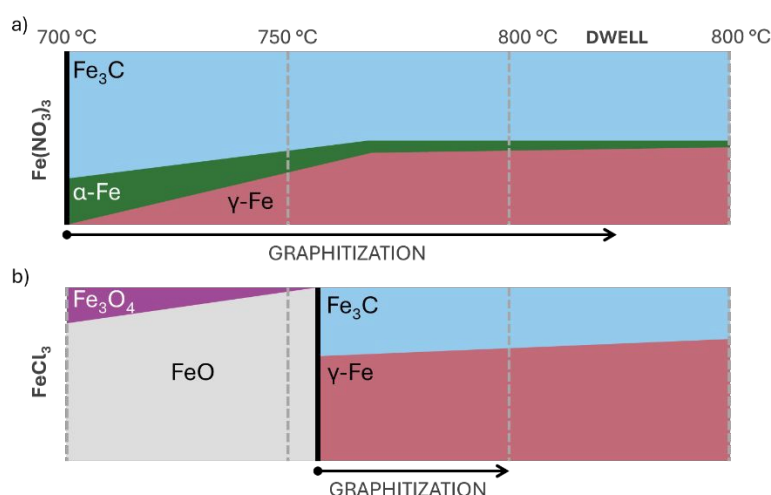
Figure 9. Schematic of the evolution of iron phases and graphitic carbon during pyrolysis of microcrystalline cellulose with a) \text{Fe}(\text{NO}_3)_3 and b) \text{FeCl}_3 from 700 °C.
