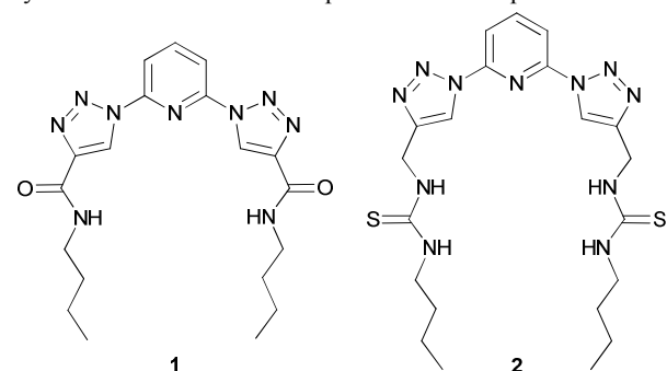
Chart 1: Previously reported 2,6-bis-(1,2,3-triazolyl)-pyridine receptors to the properties of the acyclic systems.
