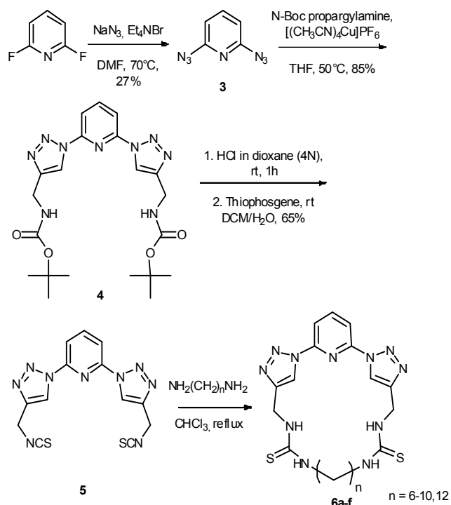
Scheme 1: Synthesis of the cyclic hosts 6a-f
