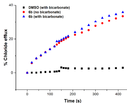
Fig. 6 Chloride efflux promoted by compound 6b (2 % molar carrier to lipid) from unilamellar POPC vesicles loaded with 450 mM NaCl buffered to pH 7.2 with 20 mM sodium phosphate salts. The vesicles were dispersed in 162 mM Na 2 SO 4 buffered to pH 7.2 with 20 mM sodium phosphate salts. At t = 120s, a solution of NaHCO 3 was added to give a 40 mM external concentration (blue markers) or the experiment was allowed to continue without the addition of NaHCO 3 (red markers). At the end of the experiment, detergent was added to lyse the vesicles and calibrate the ISE to 100 % chloride efflux. Each point represents the average of three trials.
