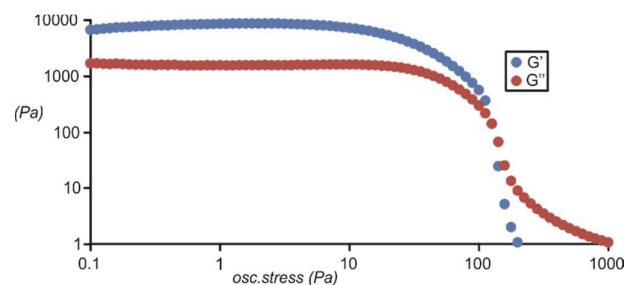
Figure 2 stress sweep rheometry for a 2% w/v gel of 1 in 1,2-dibromoethane.
