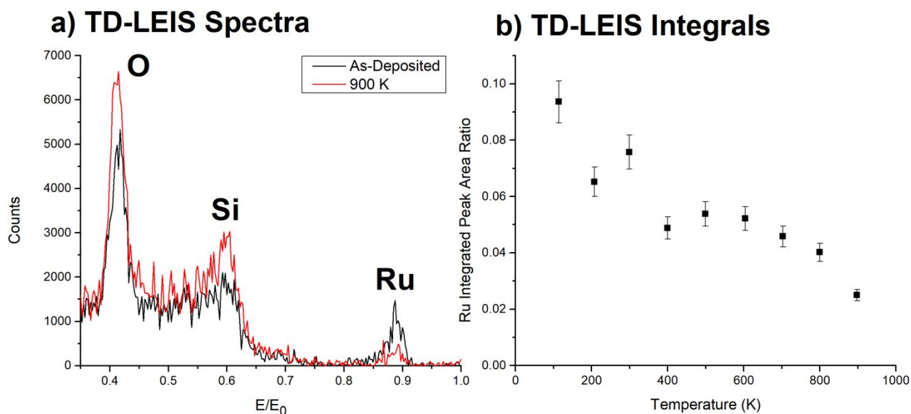
Figure 2: TD-LEIS of CS- \text{Ru}_3/\text{SiO}_2 . a) LEIS spectra for initial and final temperature measurements. b) Integrated \text{Ru}/(\text{Si}+\text{O}) peak ratio vs. temperature. Uncertainties in the Ru peak area ratios are ~8%. The sputter effects of the \text{He}^+ on the sample are discussed in the supplementary information (see Figure S14).
