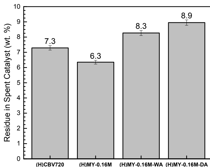
Figure 8: Residue deposits on spent catalysts using modified reactor setup. Reaction conducted at 450 °C, 1:1:PPG:Catalyst ratio, 2000 MW PPG polymer with 10-minute reaction time, under N_2 atmosphere.
