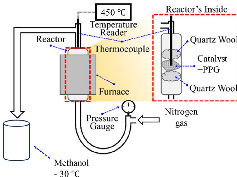
Figure 5: Process Diagram of modified reactor setup.
