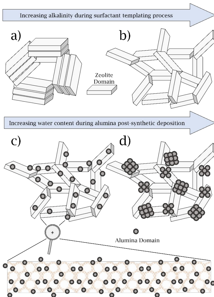
Scheme 1: Schematic representation of the MY catalysts synthesized. a) MY-0.09M, b) MY-0.16M, c) MY-0.16M-DA, d) MY-0.16M-WA.
