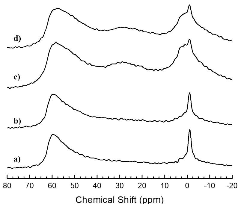
Figure 1: Solid state ^{27}\text{Al} NMR spectrum of the parent zeolite and synthesized materials; a) (H)MY-0.09M; b) (H)MY-0.16M; c) (H)MY-0.16M-WA; d) (H)MY-0.16M-DA.
