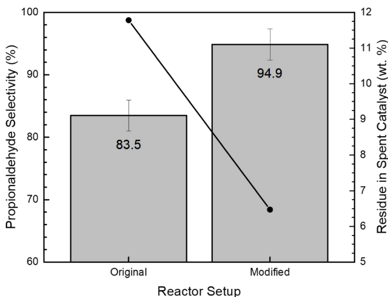
Figure 6: (Bar graph) Propionaldehyde selectivity changes over (line plot) residue deposits on spent (H)MY-0.16M material with changes in the reactor setup. Reactions conducted at 450 °C, 1:1:PPG:Catalyst ratio, 425 MW PPG polymer with 10-minute reaction time, under N 2 atmosphere.
