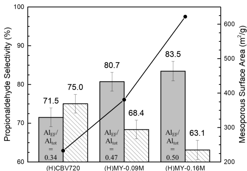
Figure 4: (Bar graph) Propionaldehyde Selectivity changes over (line plot) mesoporous surface area and Al EF content of measured catalysts. (grey) Selectivity of propionaldehyde measured with catalyst that underwent pretreatment, (dashed pattern) selectivity of propionaldehyde measured with catalyst that had no pretreatment materials, (numbers inside the bar graph) Al EF content of measured catalysts. Original reaction setup conducted at 450 °C, 1:1:PPG:Catalyst ratio, 425 MW PPG polymer with 10-minute reaction time, under N 2 atmosphere.
