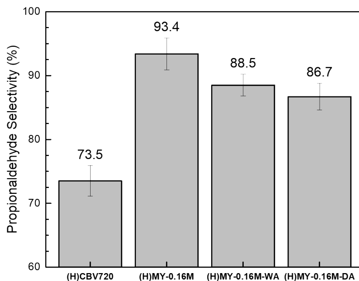
Figure 7: Propionaldehyde selectivity with measured catalyst using modified reactor setup. Reaction conducted at 450 °C, 1:1:PPG:Catalyst ratio, 2000 MW PPG polymer with 10-minute reaction time, under \text{N}_2 atmosphere.
