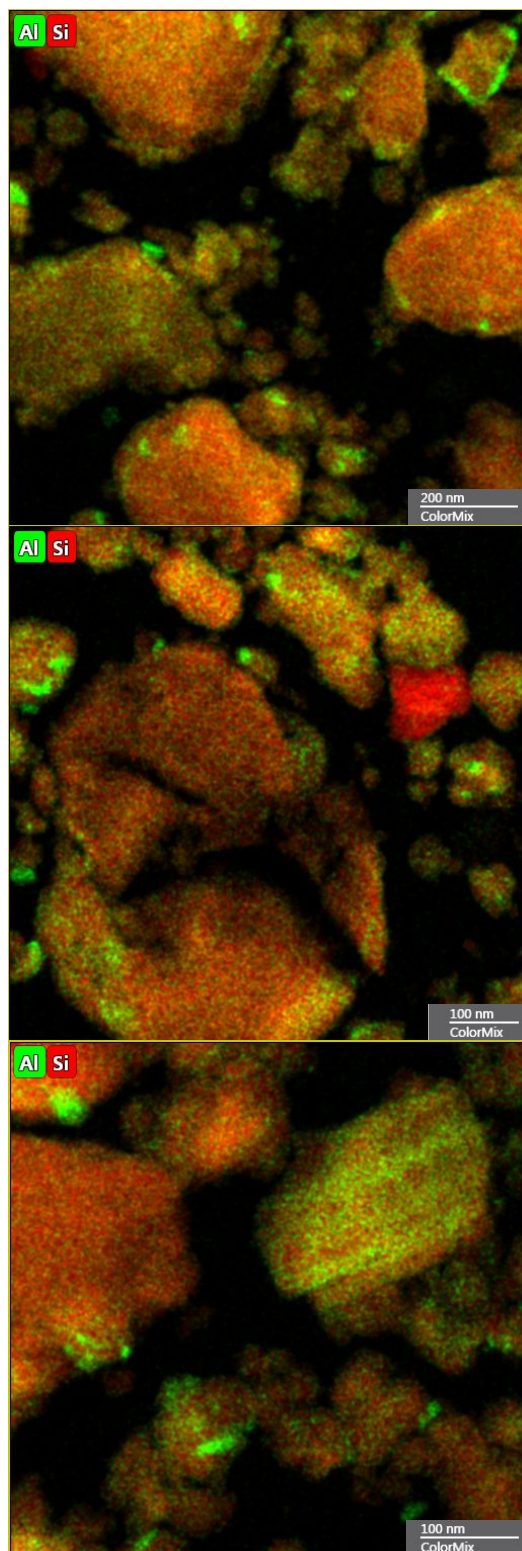
Figure 3: TEM-EDX images of microtomed MY-0.16M-DA material under different magnifications.
