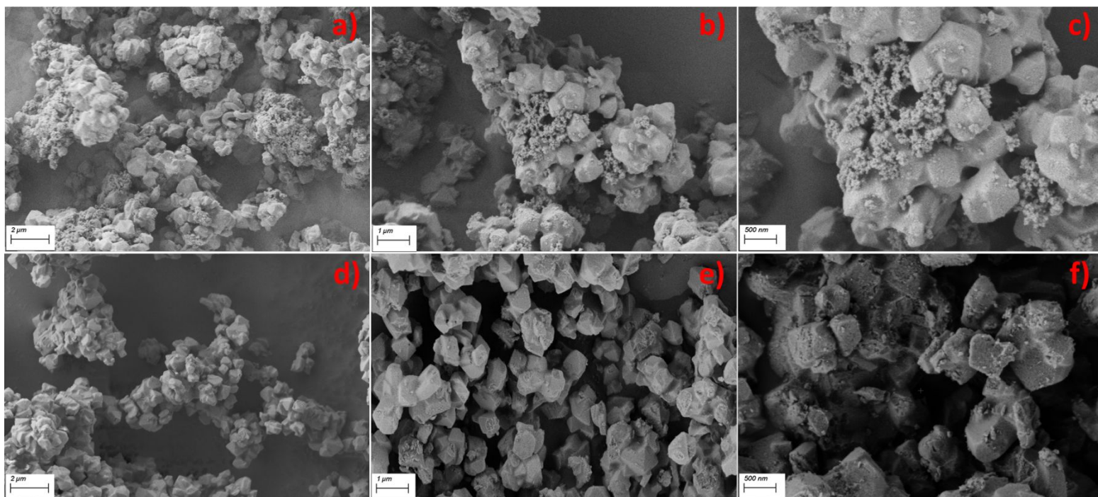
Figure 2: SEM images of alumina deposited catalysts. a-c) MY-0.16M-WA and d-f) MY-0.16M-DA.
