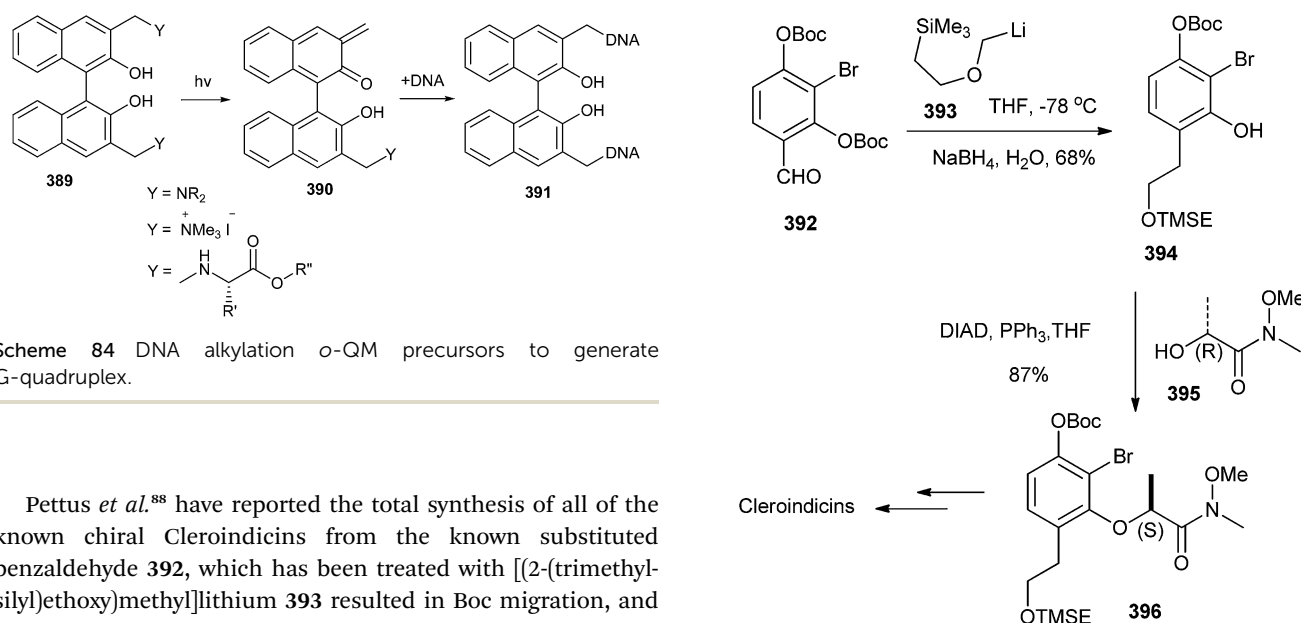
Scheme 85 Synthesis of chiral Clorindicins from the substituted benzaldehyde 392 .
