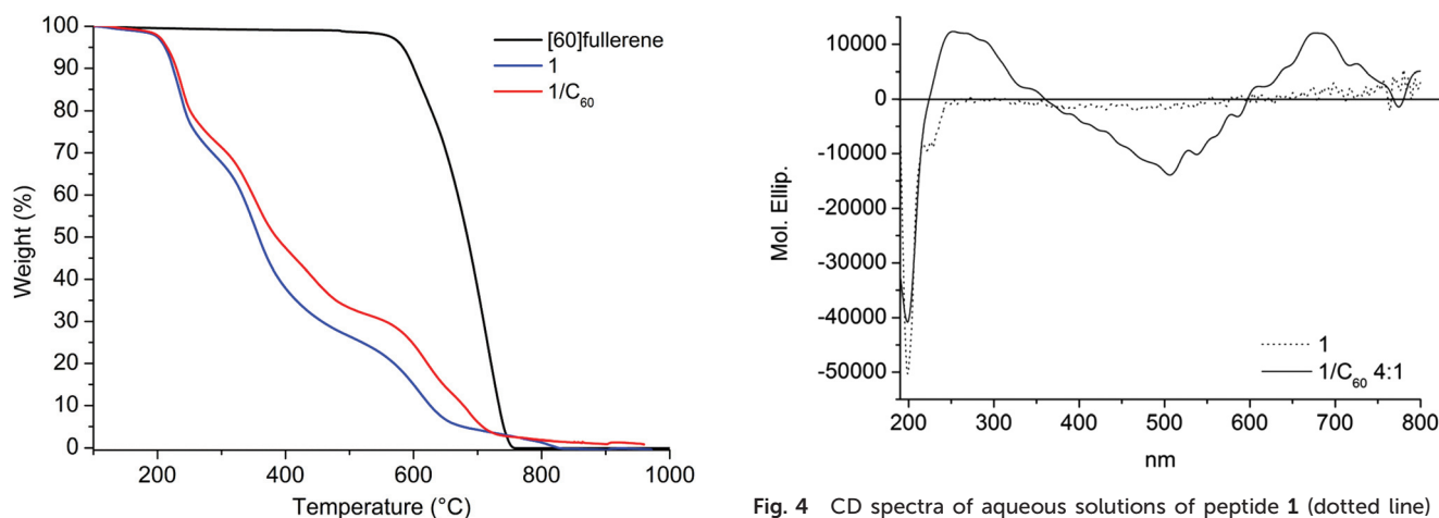
Fig. 3 TGA analysis (under a nitrogen atmosphere) of [60]fullerene, 1 and the 1/C 60 solution obtained by HSV.
