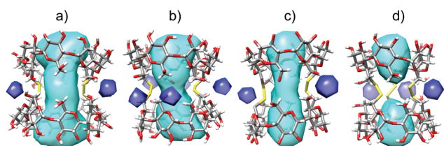
Fig. 3 Solvent accessible cavities (cyan) of duplex 7 as calculated using Surfnets. Comparison with smaller homologues. (a) \gamma -CD duplex 7 ( 740 \text{ \AA}^3 ); (b) \beta -CD duplex ( 426 \text{ \AA}^3 ); (c) \alpha -CD duplex ( 296 \text{ \AA}^3 ); (d) \alpha -CD duplex connected with three disulfide bonds ( 2 \times 114 \text{ \AA}^3 ). The dark blue-colored spots are small solvent-accessible voids outside the cavity.
