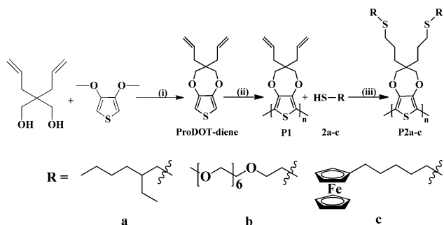
Scheme 1 Synthesis of ProDOT-diene ( 1 ), electrochemical polymerization of ( 1 ) to form poly(ProDOT-diene) ( P1 ) and “click” reaction of P1 with various thiols 2a–c to form P2a–c . (i) pTSA in toluene at 100 °C for 2 days (ii) ACN–TBAP; (iii) 0.1% DMAP, UV 365 nm, room temperature.
