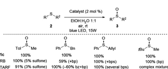
Scheme 3 Comparative study of catalyst 1c with Rose Bengal (RB) and tetra- O -acetylriboflavin (TARF) (bp = byproducts, bz = benzaldehyde) (see the ESI† for spectra).
