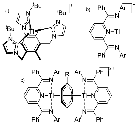
Fig. 27 Both the (a) [Tl(timtm-bu)]^+ and (b) [Tl(ArN=CPh)_2]^+ complexes derive from Tl^+[OTf]^- and are synthesized via complexation reactions of the corresponding ligands. In addition, the inverted sandwich structure (c) [Tl_2(ArN=CPh)_4]^{2+} ( Ar = 2,6-Et_2C_6H_3 , 2,5-tBu_2C_6H_3 ; R = H, Me ) was isolated.
