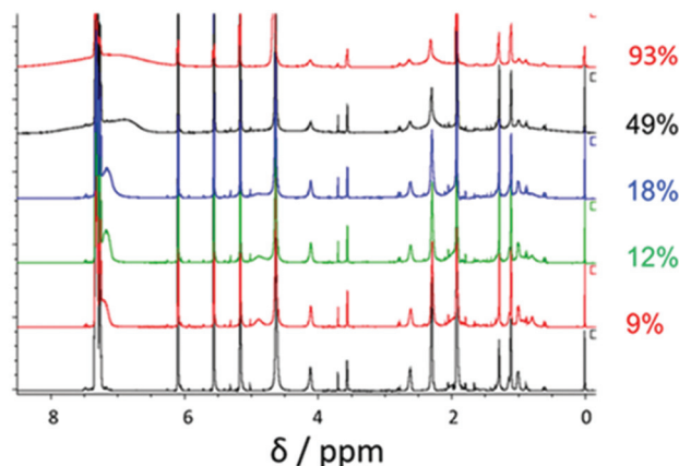
Fig. 2 ^1\text{H} NMR spectra recorded during the RAFT dispersion polymerization of BzMA at 70 °C in d_6 -ethanol targeting a final diblock composition of PDMA 43 –PBzMA 500 . Monomer conversions were calculated by comparing the integrals of the vinyl monomer to the t = 0 spectrum using TMS as the internal standard.
