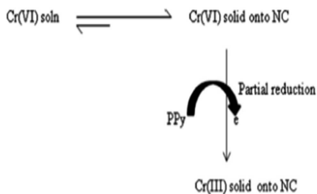
Scheme 5 The mechanism for adsorption and partial reduction of Cr(VI) onto the PPy-OMMT nanocomposite. 123
