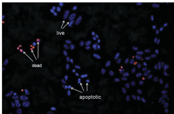
Fig. 4 Representative image that shows the morphological changes of Hep-2 cells after incubation with \{\text{Mo}_6\text{I}_8\}^{0.001}\text{@SiO}_2 ( 1.5 \text{ mg mL}^{-1} ), as detected by dual staining by Hoechst 33342/PI.
