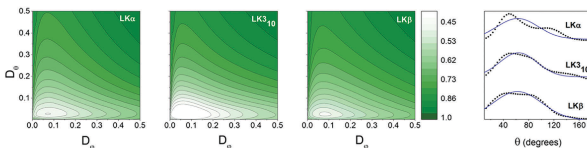
Fig. 3 Orientational information: contour plots: variation of \chi^2 with D_\phi and D_\theta for methyl groups of LK peptides at the air-water interface. D_\phi and D_\theta are inferred from the point for which the variance \chi^2 is at a minimum. Values for all three peptides may be found in Table 1. Far right: Orientation distributions of leucine methyl groups in LK peptides at the air/water interface in black. Gaussian fits are shown with blue line.
