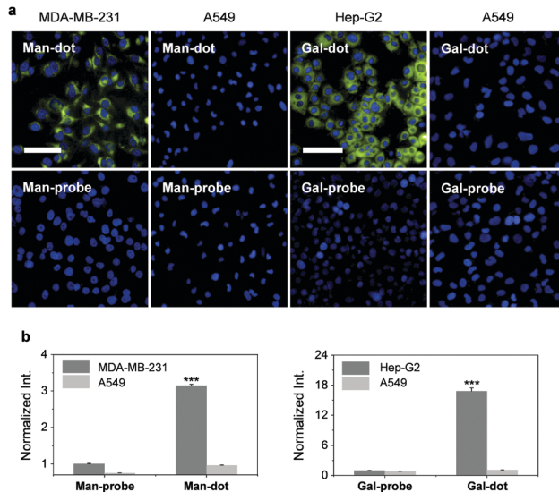
Fig. 3 Fluorescence (a) imaging and (b) quantification (***) P < 0.001 with respect to the group of glycoprobe alone for target cells) of MDA-MB-231 (human triple-negative breast cancer), Hep-G2 (human liver cancer) and A549 (human lung cancer) cells with glycoprobe alone (8 \mu\text{M} ) or glycodots (glycoprobe/poly-CD = 8 \mu\text{M} /640 \mu\text{g mL}^{-1} ). Scale bars = 100 \mu\text{m} . The excitation and emission channels used are 460–490 nm and 530–590 nm, respectively. The cell nuclei were stained by Hoechst 33342.
