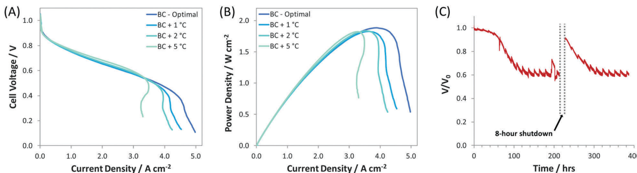
Fig. 4 (A) i - V and (B) i -power curves (10 mV s -1 forward scans) at increasing gas feed dew points for AEMFCs fabricated with the BC anode (details given in Table 1). The anode/cathode dew points for each test were: BC-optimal (45 °C/46 °C), BC + 1 °C (46 °C/47 °C), BC + 2 °C (47 °C/48 °C), BC + 5 °C (50 °C/50 °C); (C) 400 h AEMFC stability test at 600 mA cm -2 (with an 8 h cold shut down). The optimized anode/cathode dew points for the stability test were 52 °C/52 °C. For all experiments, the ETFE-BTMA membrane and AEI were used; the cell temperature was fixed at 60 °C; H 2 and O 2 were fed at flow rates of 1.0 L min -1 to the anode and cathode, respectively.
