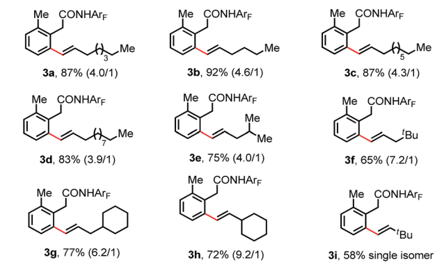
\text{1} + \text{2} \xrightarrow[\text{O}_2, \text{DCE}, 80^\circ\text{C}, 6\text{ h}]{\text{Pd(OAc)}_2 (5\text{ mol\%}), \text{L22} (10\text{ mol\%}), \text{Cu(OAc)}_2 (0.2\text{ equiv})} \text{3, linear} + \text{3', branched} \text{Ar} = 4\text{-(CF}_3\text{)}_2\text{C}_6\text{H}_3 \text{R} = \text{alkyl}
