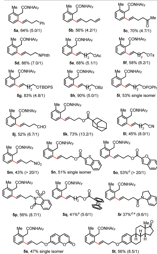
\text{Ar}_F = 4\text{-(CF}_3\text{)C}_6\text{F}_4 \text{R} = \text{alkyl} 5, linear 5', branched
