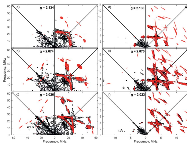
Fig. 5 X-band 4-pulse HYSCORE spectra of [\text{1}\cdot\text{H}_2]^+[\text{BAR}_4^F]^- (panels (a–c)) and [\text{1}\cdot^2\text{H}_2]^+[\text{BAR}_4^F]^- (panels (d–f)) at 2.5 mM in 7 : 1 PhMe : DFB, each collected at three field positions as indicated by g -value. The samples were frozen glasses at 20 K and measured with pulse lengths for ^2\text{H} of \pi/2 = 12 ns and \pi = 8 ns, \tau = 204 ns, initial variable delays of 100 ns and a time step of 20 ns over 300 points in both axes. The pulse lengths for ^1\text{H} were \pi/2 = 8 ns and \pi = 12 ns, \tau = 144, 140, 132 ns (top to bottom), initial variable delays of 100 ns and a time step of 8 ns, and 200 points in both axes. The microwave frequency was 9.7411 and 9.7583 GHz, respectively. Experimental data is in black, while simulations are overlaid in red.
