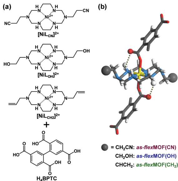
Fig. 1 (a) Square planar Ni(II) macrocycles with different pendant arms as metal building blocks and H_4BPTC as an organic building block. (b) Representation of the linear connectivity between two building units via coordinate and hydrogen bonds. Colour scheme: Ni, yellow; C, grey; O, red; N, blue; H, white.
