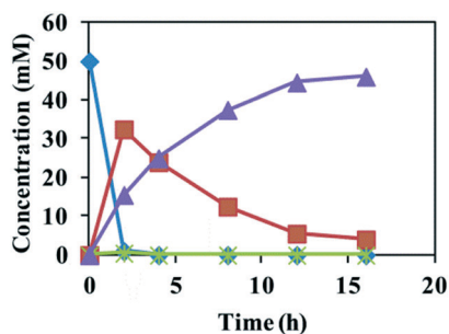
Fig. 1 Time course of the conversion of styrene oxide 1c (50 mM) to (S)- 4c with resting cells of E. coli (SpEH-BDHA-GoSCR-MVTA) (20 g cdw L -1 ) in a two-liquid phase system. ♦ = the concentration of 1c ; ■ = the concentration of 2c ; × = the concentration of 3c ; and ▲ = the concentration of (S)- 4c .
