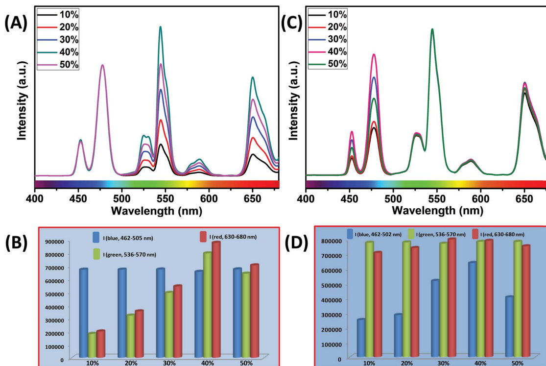
Fig. 7 (A) UCL spectra of CSS (5 mol% \text{Er}^{3+} ) UCNP samples with different \text{Yb}^{3+} concentrations in the outermost shell, where the \text{Yb}^{3+} concentration in the core remains unchanged at 40 mol%. Note that the UCL spectra are normalized to the blue ( \text{Tm}^{3+} , 462–505 nm) emission. (B) Integrated intensity of blue ( \text{Tm}^{3+} , 462–505 nm), green ( \text{Er}^{3+} , 536–570 nm) and red ( \text{Er}^{3+} , 630–680 nm) emissions of CSS UCNP samples with different \text{Yb}^{3+} concentrations in the outermost shell. Note that integrated emissions are normalized to the blue ( \text{Tm}^{3+} , 462–505 nm) emission. (C) UCL spectra of CSS (5 mol% \text{Er}^{3+} ) UCNP samples with different \text{Yb}^{3+} concentrations in the core, where the \text{Yb}^{3+} concentration in the outermost shell remains intact at 40 mol%. Note that the UCL spectra are normalized to the green ( \text{Er}^{3+} , 536–570 nm) emission. (D) Integrated intensity of blue ( \text{Tm}^{3+} , 462–505 nm), green ( \text{Er}^{3+} , 536–570 nm) and red ( \text{Er}^{3+} , 630–680 nm) emissions of CSS UCNP samples with different \text{Yb}^{3+} concentrations in the core. Note that integrated emissions are normalized to the green ( \text{Er}^{3+} , 536–570 nm) emission.
