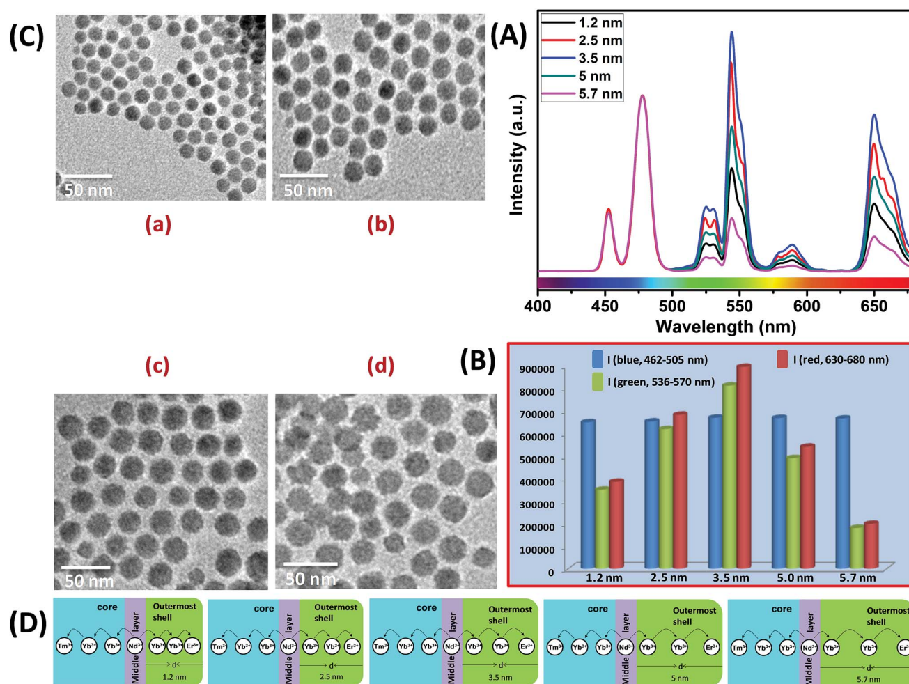
Fig. 4 (A) UCL spectra of CSS UCNPs (5 mol% \text{Er}^{3+} ) with different thickness of the outermost shell over CS (30 mol% \text{Nd}^{3+} ) UCNPs ( d = 1.2–5.7 \text{ nm} ). (B) Integrated intensity of blue ( \text{Tm}^{3+} , 462–505 nm), green ( \text{Er}^{3+} , 536–570 nm) and red ( \text{Er}^{3+} , 630–680 nm) emissions of CSS UCNPs with different outermost shell thickness ( d = 1.2–5.7 \text{ nm} ). Note that, the UCL spectra and integrated emissions in (A) and (B), respectively, are normalized to the blue (462–505 nm) emission. (C) TEM images of CSS (5 mol% \text{Er}^{3+} ) UCNPs with different outermost shell thickness ((a) 1.2 nm, (b) 2.5 nm, (c) 5.0 nm and (d) 5.7 nm). (D) Mechanistic investigation of interfacial ET from the \text{Nd}^{3+} -containing middle shell layer to the \text{Tm}^{3+} -containing core (with defined shell thickness d = 2.5 \text{ nm} ) and \text{Er}^{3+} -containing outermost shell (with different shell thickness d = 1.2–5.7 \text{ nm} ) in CSS (5 mol% \text{Er}^{3+} ) UCNPs.
