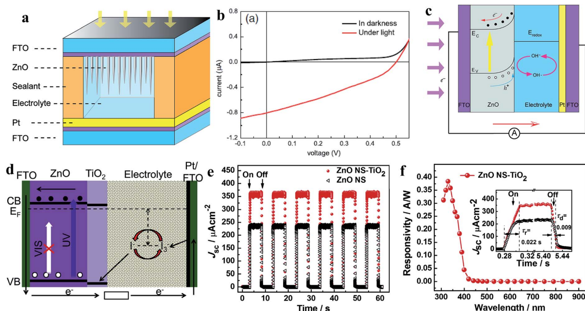
Fig. 16 ZnO NN photoanode: (a) device schematic of ZnO NN photoanode-based PECC-type PD. (b and c) I - V profiles in dark and UV ( 365 \text{ nm} , 1.25 \text{ mW cm}^{-2} ) conditions and self-powered working mechanism under exposure to UV, respectively. Reproduced with permission from ref. 209 Copyright 2013 Springer. ZnO NSs-TiO 2 core-shell photoanodes: (d) energy band diagram and working principle of the PD under exposure to UV irradiation. (e) Cyclic photoresponses of ZnO NSs-TiO 2 core-shell photoanode- and ZnO NSs photoanode-based PDs upon exposure to UV light ( 365 \text{ nm} , 20 \text{ mW cm}^{-2} ) in the off and on states. (f) Spectral photoresponse and inset response/recovery time calculation of the PECC PD. Reproduced with permission from ref. 210 Copyright 2013 Elsevier.
