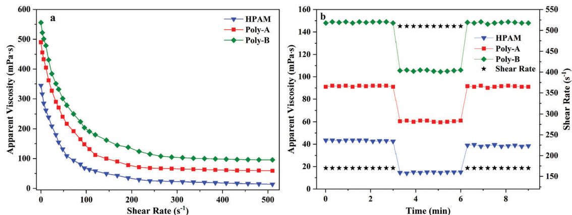
Fig. 6 (a) Shear thinning behavior of the copolymers and (b) shear recovery of the copolymers.
