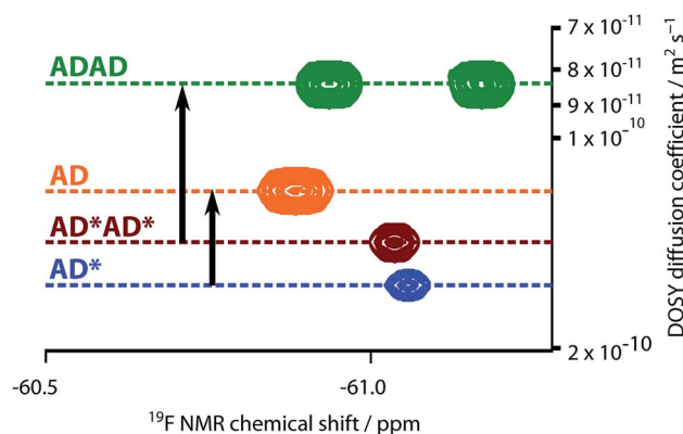
Fig. 7 Overlay of the {}^{19}\text{F} NMR DOSY (400 MHz, TCE- d_2 , 298 K, ca. 5 mM) spectra of AD, AD*, ADAD, and AD*AD*. Arrows highlight the decrease in the diffusion coefficient due to intermolecular hydrogen bonding interactions involving the phenols in AD and ADAD. In AD*AD*, the two {}^{19}\text{F} signals are not resolved.
