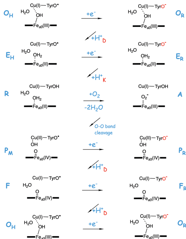
Fig. 9 Suggested reaction mechanism during enzyme turnover for the \text{aa}_3 A family oxidases, showing that the initial electron transfer to the BNC reduces the tyrosyl radical into tyrosinate in every reduction step. The channel suggested to be used for the following proton uptake is indicated with a D or K subindex on the protons. 36 The electronic structure of the activated \text{E}_\text{H} state has a fraction of tyrosinate plus \text{Fe}(\text{III}) mixed in.
