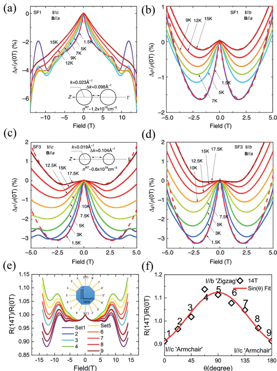
Fig. 12 Negative MR in the SF1 sample for (a) I/c and (b) I/b at different temperatures, respectively. The low field MR in the SF3 sample at different temperatures when (c) I/c and (d) I/b . The low-field negative MR in the SF1 sample is more anisotropic than the SF3 sample. The insets of (a) and (c) show the sketches of the cross-sections of Fermi surfaces for the SF1 and SF3 samples, respectively. (e) Anisotropic MR for I applied along various directions and B//a . (f) The normalized MR curves by the zero-field resistivity for better comparison. Note the exotic non-saturating behavior up to 14 T for I/c -axis. Reproduced from ref. 162 with permission from Nature Publishing Group.
