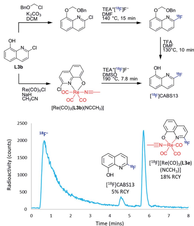
Fig. 5 (Top) Alternative radiosynthesis of [^{18}\text{F}]\text{CABS13} via the rhenium(i) complexation–dissociation method circumvented multiple-step synthesis, as reported by Liang, et al. 34 (Bottom) Radiochromatogram depicting the formation of [^{18}\text{F}]\text{CABS13} in 5% RCY from the thermal dissociation of [^{18}\text{F}][\text{Re}(\text{CO})_3(\text{L3e})(\text{NCCH}_3)] which formed in 18% RCY.
