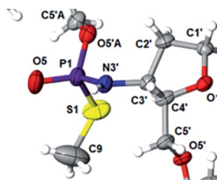
Fig. 1 Crystal structure of DMT dG^iBu NPSMe T_{OAc} 10f showing partial structure and spatial orientation of substituents around the phosphorus stereogenic center (marked P1). Compound 10 was obtained from the monomer 6Gf (fast-eluting 5'- O -DMT-3'-amino-2',3'-dideoxy-N6-iBu-guanosine-3'- N -(2-thio-4,4-pentamethylene-1,3,2-oxathiaphospholane). The oxygen atom marked O5'A belongs to the thymidine residue.
