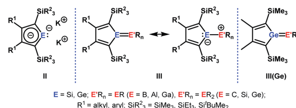
Scheme 1 Dipotassium sila- or germacyclopentadienediides II , polarised heteroalkenes I and products III and III(Ge) .
