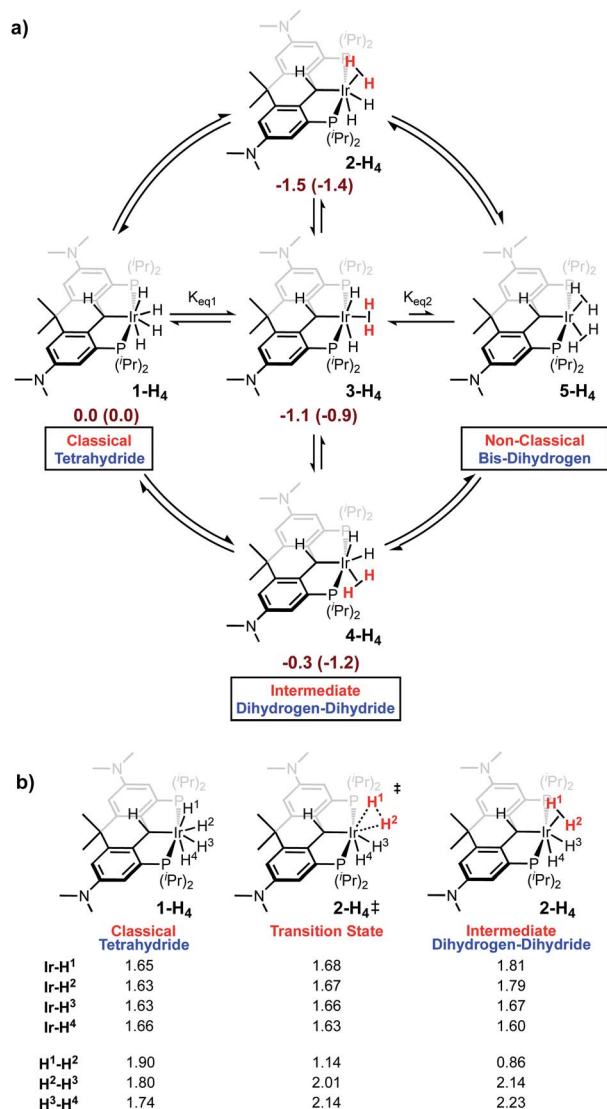
Scheme 2 (a) Outline of isomerism in \text{Ir-H}_4 with benzene-solvated enthalpies (Gibbs energies) in \text{kcal mol}^{-1} (b) Ir-H and H-H distances ( \text{\AA} ) found in M06 DFT structures.
