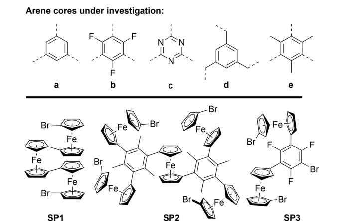
Scheme 1 (Top) Preparation of tris-phosphanes 1a–d and complexes [(1a–c)E] . (II) Pd precatalyst, THF, r. t.; (III) n BuLi, Ph 2 PCL, THF, –80 °C to r. t.; (III) [E]·X ([E]·X = BH 3 ·SMe 2 or [AuCl(tht)]), CH 2 Cl 2 , r. t.; (Bottom) crystallographically characterised side products obtained during the syntheses of 4d (SP1), 4e (SP2), and 4b (SP3). For their solid-state structures, see Fig. S3.†
