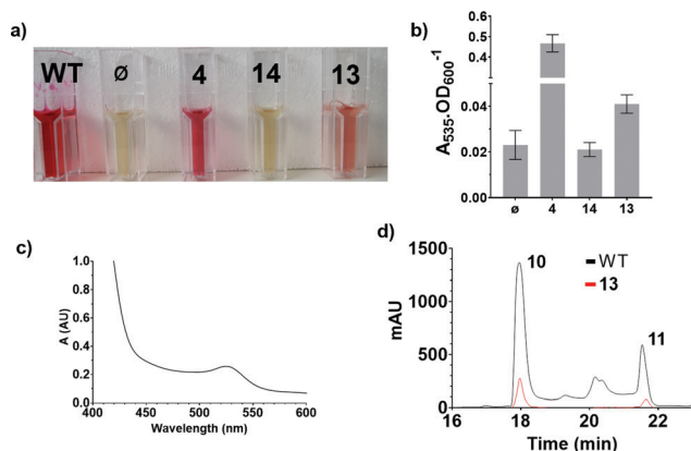
Fig. 4 Results of the quantitative chemical complementation assays; (a) ethanol extract of cultures of S39006 WT and S39006 \Delta pigD incubated with no additive ( \emptyset ), aldehyde 4 , carboxylic acid 14 or thioester 13 ; (b) Absorbance at 535 nm normalised by OD 600 for the specified extracts; (c) UV spectrum of the extract of S39006 \Delta pigD inoculated with thioester 13 ; (d) Comparison of the HPLC traces (535 nm) of the extracts of S39006 WT and S39006 \Delta pigD incubated with thioester 13 .
