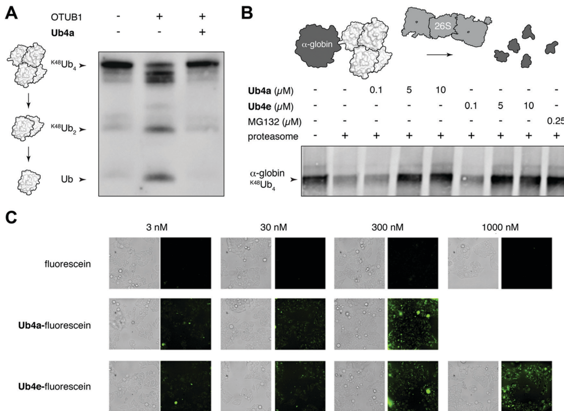
Fig. 3 Cyclic peptides inhibit Ub-dependent proteolysis and can enter cells. (A) Cyclic peptide Ub4a (2 μM) inhibits the cleavage of K^{48}Ub_4 (2 μM) by the K^{48} -specific DUB OTUB1 (0.25 μM) in vitro . Western blot with anti-Ub antibody. (B) Cyclic peptides Ub4a and Ub4e inhibit degradation of K^{48}Ub_4 -tagged HA-tagged \alpha -globin (5 μM) by the 26S proteasome (150 nM) in vitro . Similar inhibition of degradation is observed in the presence of direct proteasome inhibitor MG132. Western blot with anti-HA antibody. (C) Cyclic peptides Ub4a and Ub4e , fluorescein labelled, are internalized by live HeLa cells.
