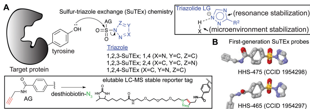
Fig. 3 Sulfur–triazole exchange (SuTEEx) chemistry. Sulfonyle-triazoles represent a new class of electrophiles that facilitate covalent reaction with tyrosines and lysines through a nucleophilic substitution reaction that is facilitated by a triazolide leaving group (LG). Both intrinsic (resonance stabilization) and extrinsic factors (protein microenvironment) are proposed to contribute to the LG ability of the triazole. Triazole regioisomers (1,2,3- and 1,2,4-isomers) can serve as the LG for development of SuTEEx ABPs. The AG of SuTEEx ABPs contains an alkyne group for CuAAC conjugation with desthiobiotin-azide to produce a LC-MS stable reporter tag. The selection of a desthiobiotin affinity handle allows enrichment and release of ABP-modified peptides from avidin-agarose beads during preparation of proteomes for LC-MS studies. (B) Crystal structures of first-generation SuTEEx ABPs HHS-475 and HHS-465, which differ by the triazole regioisomer selected as the LG.
