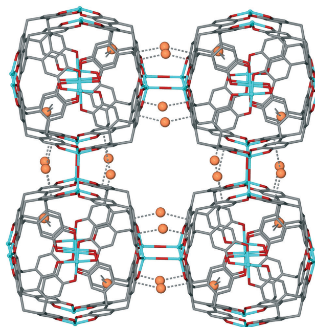
Fig. 10 3D coordination polymer of [\text{Mn}_6(\text{OH})_3(\text{ctc})_4]\cdot\text{Cs}_{10}\text{Na}_5(\text{H}_2\text{O})_n with water and Cs/Na positions inside the [\text{Mn}_6(\text{ctc})_4] cage excluded. Disordered bridging OH is shown in averaged position, and \text{Cs}^+\cdots\pi interactions as dashed lines. 22
