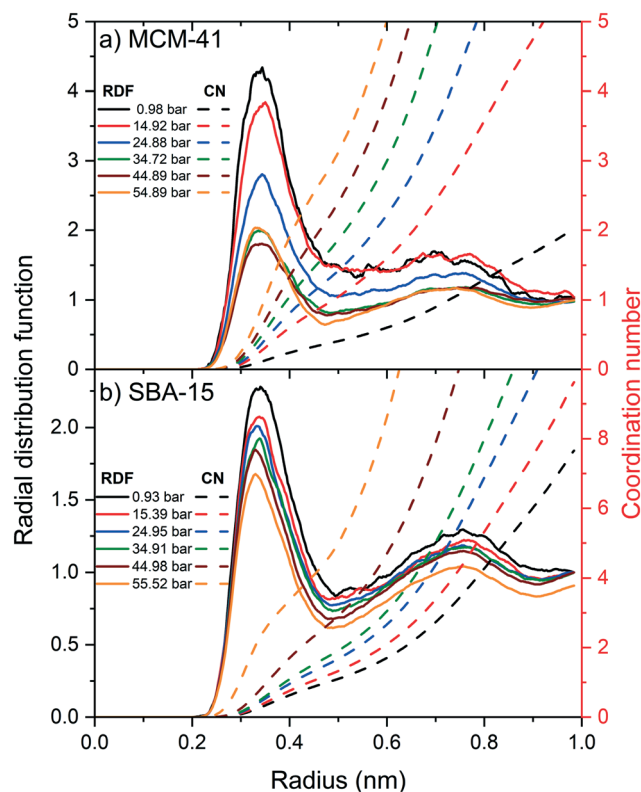
Fig. 8 The radial distribution functions and the corresponding coordination numbers of -\text{OH}-\text{C}_{60} in the MCM-41 (a) and SBA-15 (b) as a function of the applied pressure are shown. The simulation data are averaged over the last 10 ns of the simulation time.
