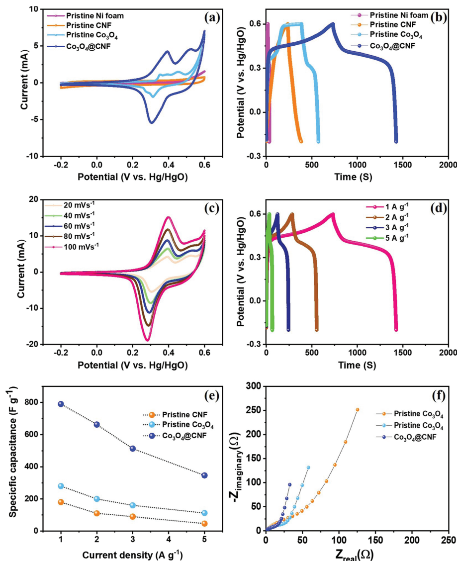
Fig. 5 Comparison of three electrode electrochemical measurements for the pristine \text{Co}_3\text{O}_4 nanoparticles, pristine CNF and 1D \text{Co}_3\text{O}_4@\text{CNF} : (a) CV curve at 20 \text{mV s}^{-1} of scan rate, (b) GCD curve of 1 \text{A g}^{-1} of current density, (c and d) CV and GCD curves at various scan rates and current densities, (e) specific capacitance and (f) EIS measurement.
