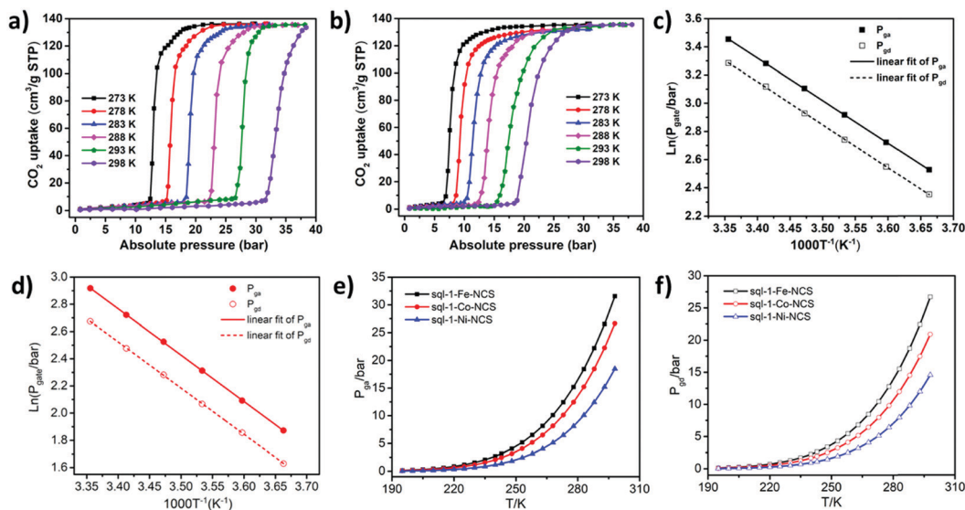
Fig. 3 High-pressure CO 2 sorption isotherms of (a) sql-1-Fe-NCS and (b) sql-1-Ni-NCS . The linear fit of gate sorption pressure ( \ln P ) and temperature ( 1000 T^{-1} ) using the Clausius–Clapeyron equation for (c) sql-1-Fe-NCS and (d) sql-1-Ni-NCS . (e) Calculated P_{\text{ga}} and (f) P_{\text{gd}} for sql-1-M-NCS (M = Fe, Co, and Ni).
