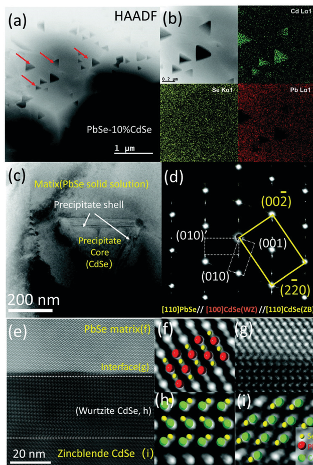
Fig. 14 Scanning and transmission electron microscopy (S/TEM) images of \text{PbSe-CdSe} sample. (a) High-angle annular dark field image showing the embedded triangular nano-precipitates in the matrix. (b) Energy-dispersive X-ray spectroscopy (EDS) mapping. (c) TEM image showing a core-shell precipitate in the matrix. (d) Selected area diffraction (SAED) pattern taken along the [110] zone axis, which reveals the interface is the wurtzite \text{CdSe} phase. (e) High-resolution STEM image with a HAADF mode image showing the core-shell sections of \text{CdSe} with \text{PbSe} matrix. (f–i) Show the atomic stacking of the matrix, interface between the matrix and shell, the shell, and core of the precipitate. Reproduced with permission from ref. 162, Copyright 2020 Royal Society of Chemistry.
