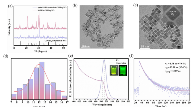
Fig. 3 (a) The XRD patterns of CsPbBr 3 PNCs synthesized by two methods; (b and c) TEM images of NADES-CsPbBr 3 PNCs. Inset in (c) shows the corresponding HRTEM image; (d) size distribution of NADES-CsPbBr 3 PNCs; (e) absorption and PL spectra of NADES-CsPbBr 3 PNCs. Inset in (e) shows the photograph of NADES-CsPbBr 3 PNCs under daylight (left) and under UV light (right); (f) the decay curve of NADES-CsPbBr 3 PNCs.
