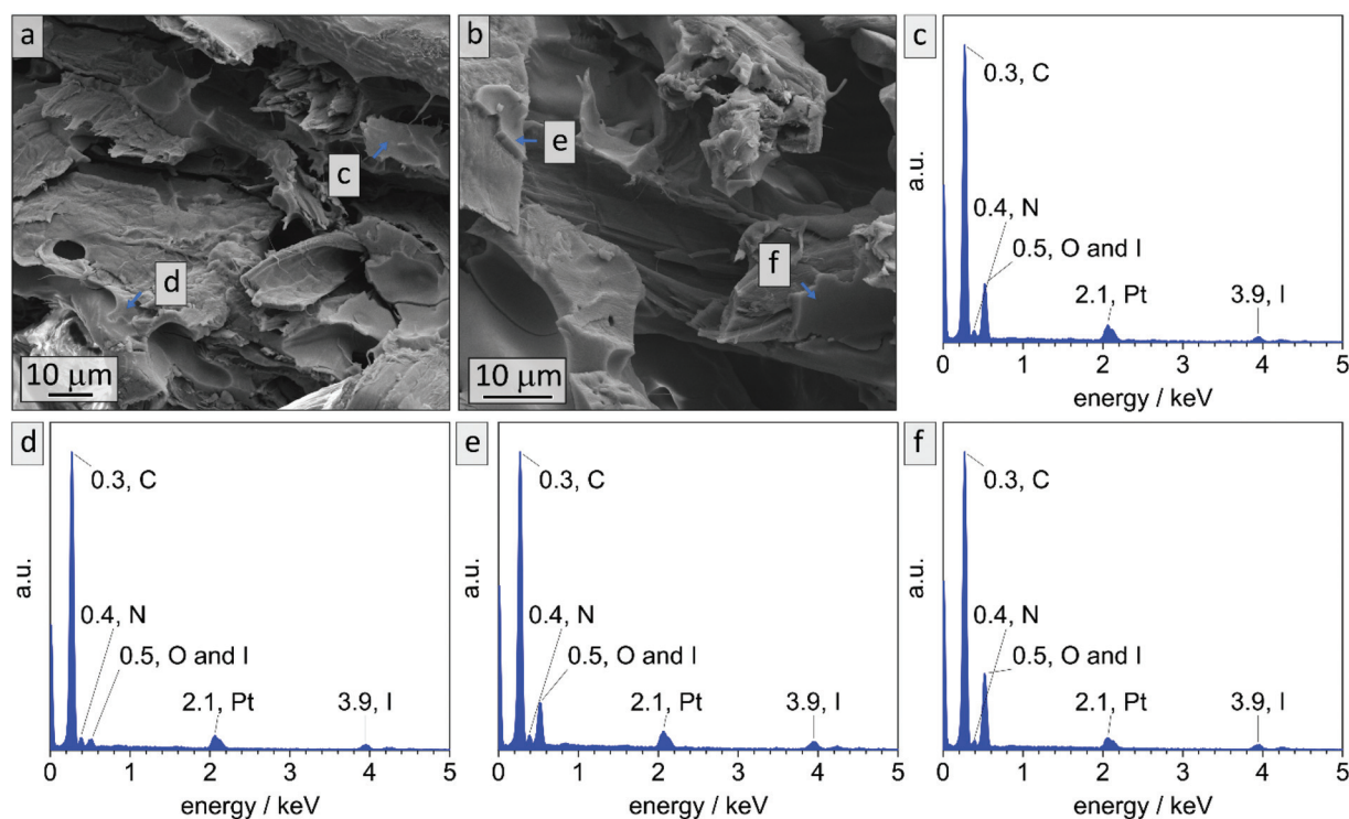
Fig. 10 EDS data collected on composite sample made of \text{PI}_{35}\text{-}b\text{-P2VP}_{65} 186 on cellulose substrate via vertical deposition after stabilization with DIB. (a and b) Cross-sectional SEM images and exemplary locations of EDS point spectra (c–f) are marked.
