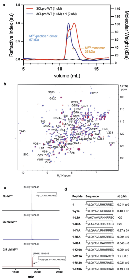
Fig. 4 (a) SEC-MALLS of SARS-CoV-2 M^{Pro} with and without peptide 1. SARS-CoV-2 M^{Pro} (red line) exists in equilibrium between monomeric and homodimeric forms giving rise to two peaks (in ca. 1 : 1.25 ratio of monomer to dimer) in the size-exclusion chromatogram at a concentration of 1 \mu M in aqueous buffer (50 mM Tris-HCl pH 8.0, 150 mM NaCl). MALLS analysis indicates an approximate molecular weight of 36 kDa for the monomer (calculated molecular weight = 33.8 kDa). After addition of two molar equivalents of 1, M^{Pro} converges predominantly to a homodimer (blue line) with a MALLS reading of 66 kDa (calculated MW of SARS-CoV-2 M^{Pro} dimer = 67.6 kDa, MW of peptide 1 = 1874 Da) indicative of formation of the SARS-CoV-2 M^{Pro} homodimer upon binding 1. (b) Cyclic peptide inhibitor 1 binds to the dimeric form of SARS-CoV-2 M^{Pro} . Overlay of projections onto the ^{15}N - ^1H plane of 3D TROSY-HNCO spectra of 0.3 mM solutions of ^{15}N / ^{13}C / ^2H -labelled wild-type M^{Pro} . Blue and red contour lines show the spectra recorded in the absence and presence of equimolar inhibitor 1, respectively. Assignments are shown for peaks that shift or disappear in response to the inhibitor. (c) Monitoring of the cleavage of cyclic peptide inhibitor 1 with SARS-CoV-2 M^{Pro} . MALDI-TOF mass spectrum of cyclic peptide 1 (top spectrum). Negligible cleavage of 1 was observed following incubation with SARS-CoV-2 M^{Pro} under standard assay conditions (25 nM SARS-CoV-2 M^{Pro} , 5 \mu M 1, 20 mM Tris-HCl pH 7.6, 100 mM NaCl, 1 mM DTT, 1 mM EDTA) for 1 h at 37 ^{\circ}C (middle spectrum). Slow cleavage of 1 was observed (ca. \sim 30% after 1 h) in the presence of a high concentration of SARS-CoV-2 M^{Pro} to 2.5
