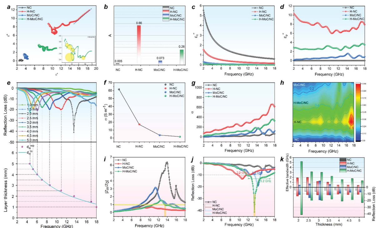
Fig. 3 The attenuation and impedance matching analysis. (a) Cole–Cole semicircle of H-MoC/NC (insert) in \varepsilon' - \varepsilon'' curves. (b) Calculated A values. (c) Calculated \varepsilon_c'' values. (d) Calculated \varepsilon_p'' values. (e) Experimental and theoretical fitted d_m values. (f) Conductivity. (g) Attenuation coefficient. (h) Dielectric loss. (i) Impedance matching plots. (j) The effective absorbing band (<−10 dB) in RL plots. (k) Effective bandwidth and minimum RL values.
