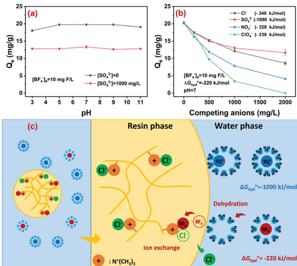
Fig. 5 Effects of pH with and without 1000 \text{ mg L}^{-1} sulfate (a) and effects of competing anions at \text{pH} = 7 (b) on the adsorption of D201 toward \text{BF}_4^- ( 10 \text{ mg-F/L} ) at 298 \text{ K} , and the plausible mechanism for \text{BF}_4^- removal (c).
