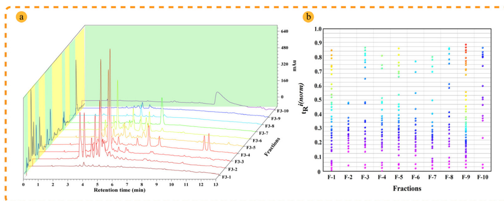
Fig. 2 Orthogonality evaluation of the established 2D chromatography system. (a) Separation effect of T. wilfordii extract in 2D RP x SFC system; (b) 2D separation orthogonality plan of RP x SFC.
