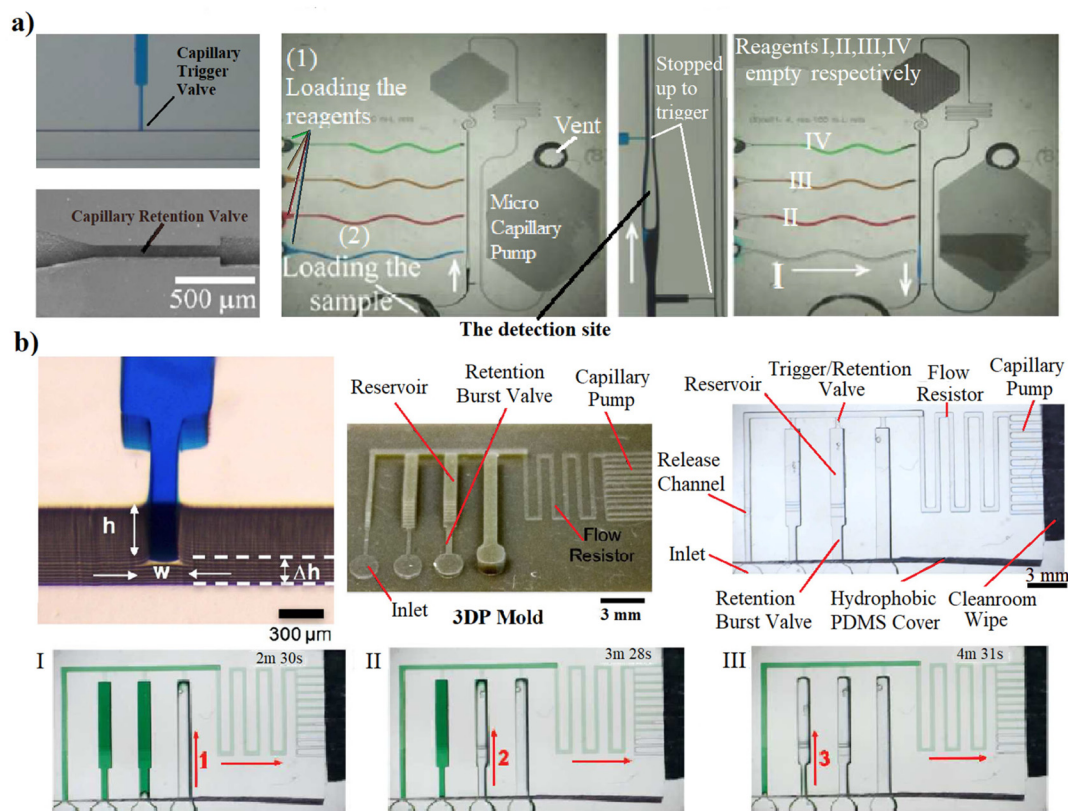
Fig. 4 Passive actuations based on combination of the upstream constriction (retention valves) and the downstream expansion (trigger valves). (a) A passive circuit that encodes sequential activation of 4 solutions. When sample reached the capillary pump, four different reagents were released based on a retention pressure. 25 (b) An autonomous capillary circuit replicated from 3D-printed mold that pre-programmed the reagents' releases by a combination of the trigger valve and the retention burst valve. Releasing liquid from its reservoir happens by reaching the burst pressure at the junction to compel the upstream retention. 18
